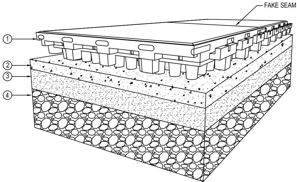
ISOMETRIC VIEW
