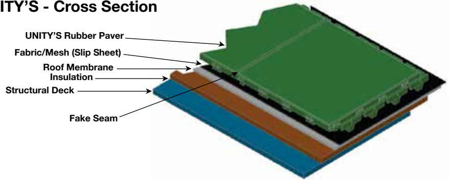
UNITY'S - Cross Section
