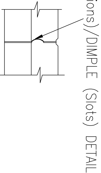
JOINT DETAIL AT PIMPLE (Projections)/DIMPLE (Slots)
