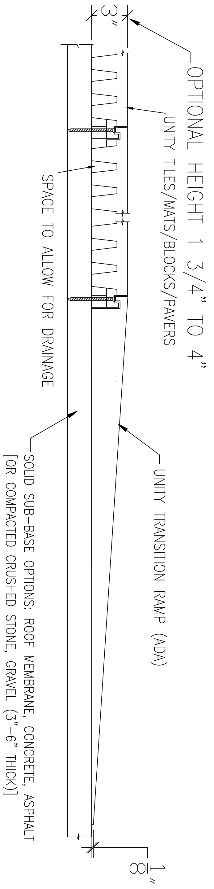
SUB-SURFACING/BASE OPTIONS - RAISED SURFACE W/ TRANSITION
