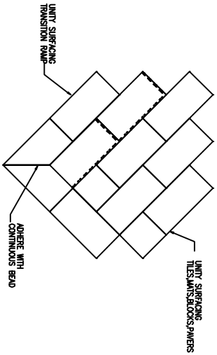
OUTSIDE CORNER TRANSITION RAMP DETAIL (POST CONSTRUCTION)
